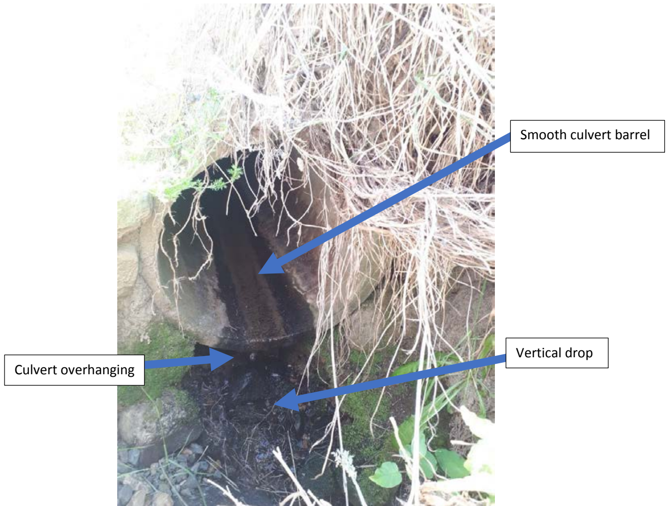
Figure E-15: Fish passage will be impeded by the fall height and undercut at the culvert outlet. The smooth culvert barrel will also lead to higher water velocities and limit fish movements under higher flows. Credit: Megan Brown.
