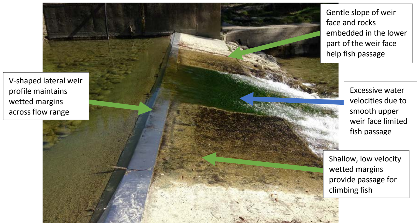
Figure E-19: An example of a crump weir used for hydrological gauging. Fish passage was impeded for swimming fish at this weir by the high water velocities. Climbing fish were able to use the wetted margins on each side of the weir to pass. Credit: Paul Franklin.
