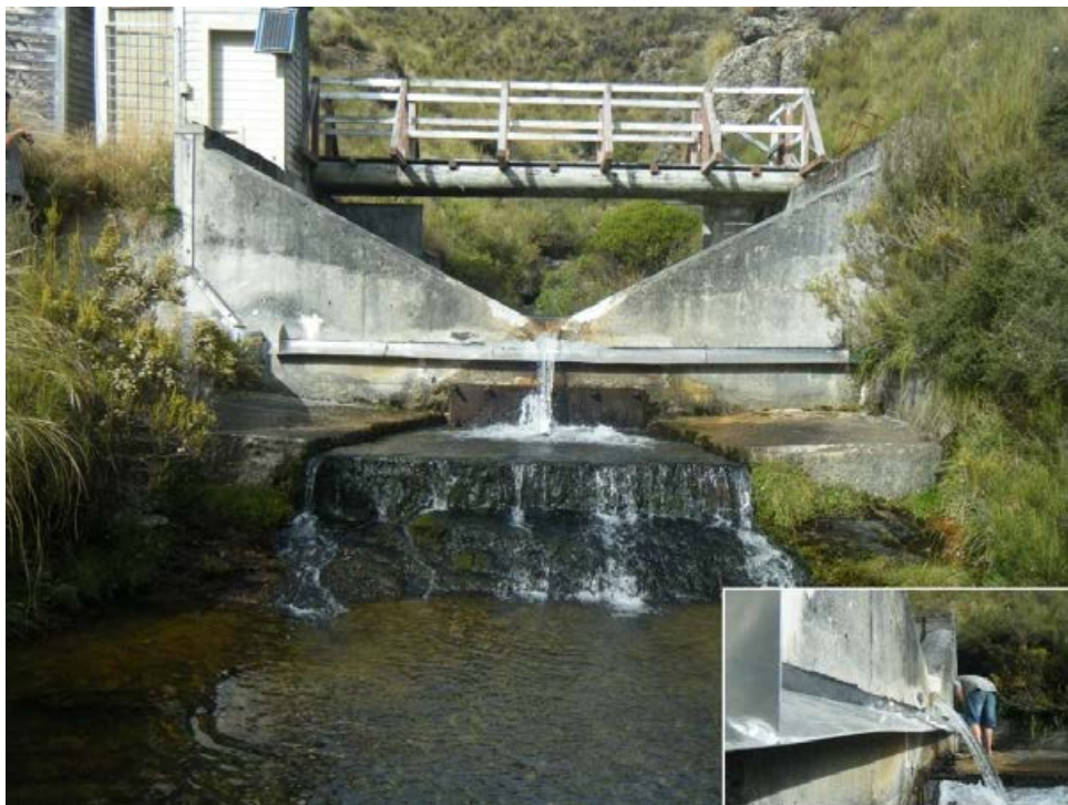
Figure 6-6: Built barrier installed in an un-named tributary of Upper Waipori River. The objective was to prevent trout and kōaro access to a key dusky galaxias stronghold in Otago. Inset shows a close-up view of the successful kōaro lip barrier. Credit: Josh Tobak.
