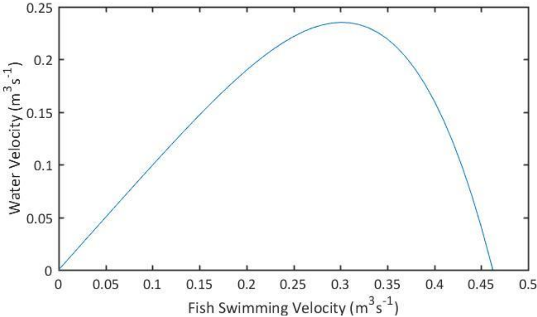
Figure 4-6: Example of a curve describing the swimming speeds required for a 5 cm inanga to successfully pass a 10 m fishway. Based on data from Nikora et al. (2003) for tests conducted at 16 – 22 °C.
